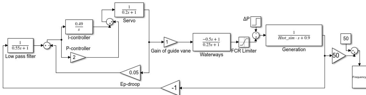
Figure 1. European power system Simulink model
