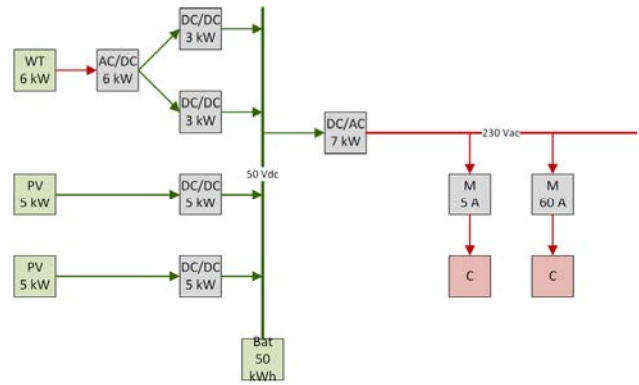
Figure 3: Block diagram of the Ndeda mini-grid power system (WT: wind turbine; PV: solar panels; M: meters; C: customers).
