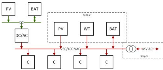
Figure 4: Block diagram of the proposed scalable mini-grid concept with an interconnection to a larger power system (WT: wind turbine; PV: solar panels; BAT: battery; C: customers).
